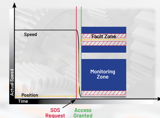
Stop Functions – Safe Operating Stop
