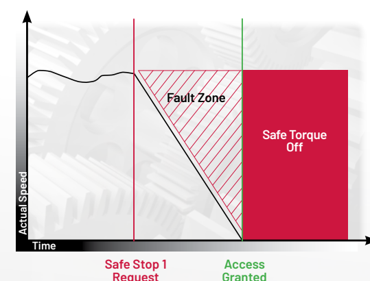
Stop Functions – Safe Stop 1
